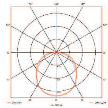
Polar Curve: Photometric data is available online for dialux and relax.
